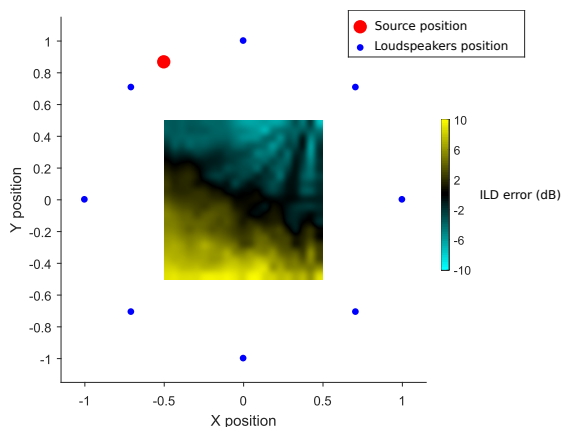
Figure 3: ILD cartography simulated using HOA spatialization method, octophonic display, and source at 30^\circ .
