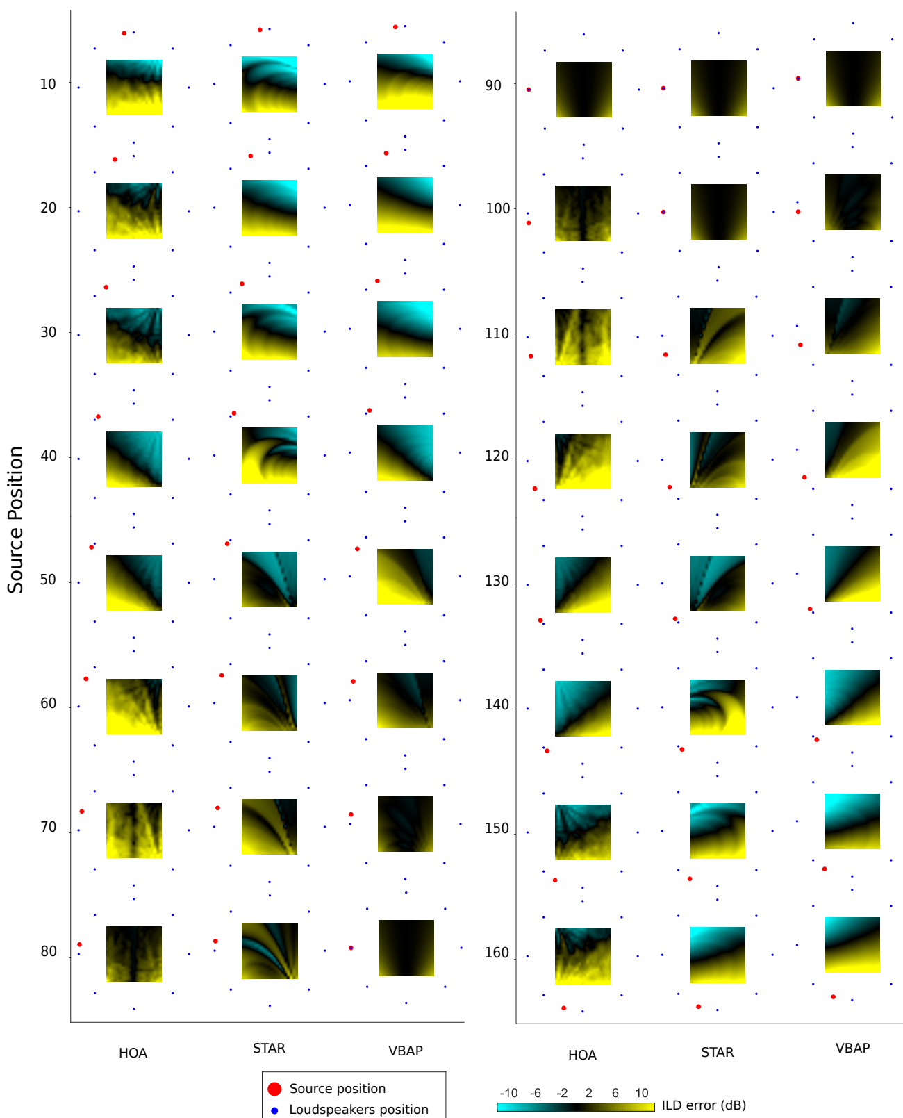
Figure 6: ILD error cartography for all spatialization methods and different source positions (azimuth from 10° to 160° by steps of 10°).
