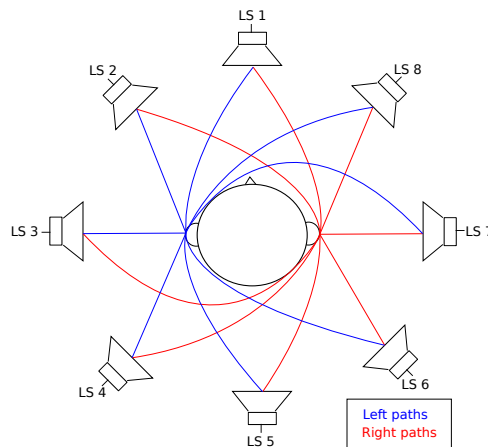
Figure 1: Acoustic paths for the octophonic configuration.
