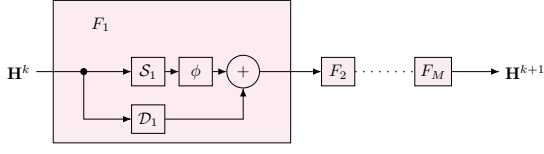
Figure 1: Block diagram showing the recurrent cell of the FRNN structure (dependencies of \mathbf{H} on discrete time index k are denoted in the superscript for brevity).
